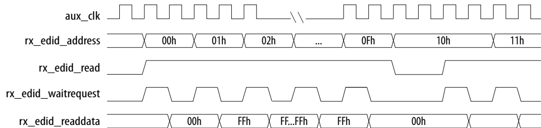
Figure 35. rx_edid Interface
